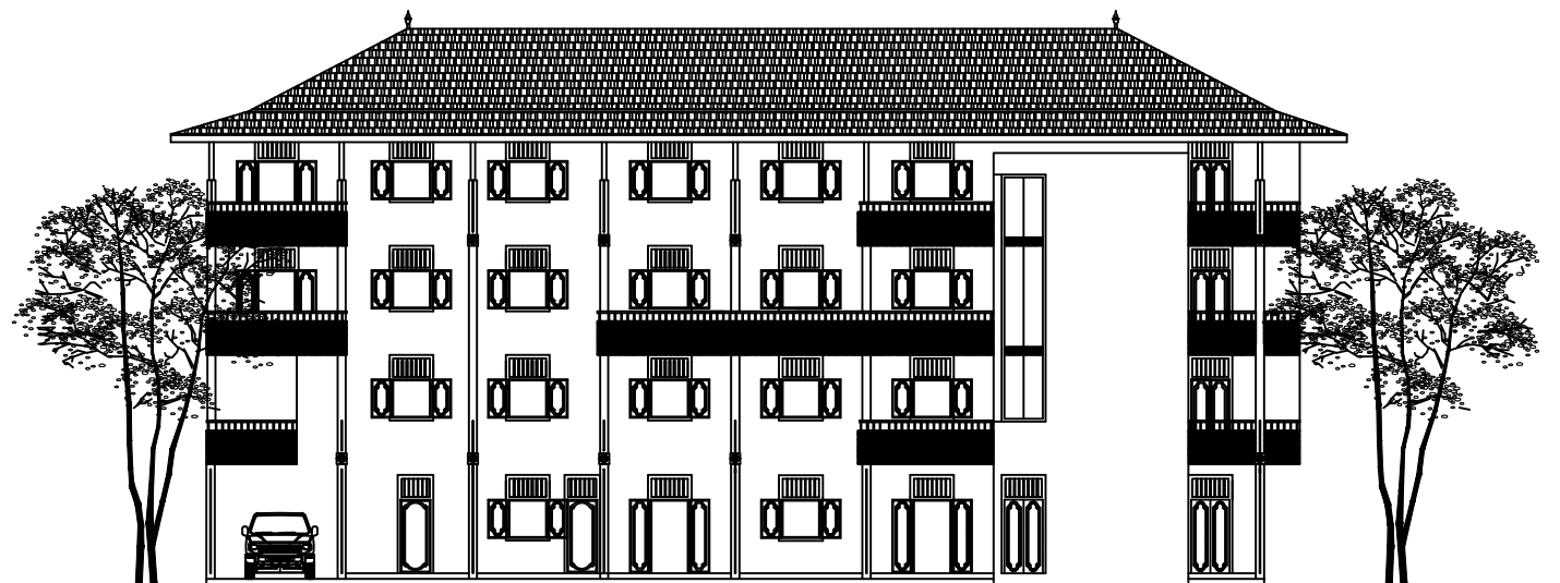
FRONT ELEVATION
