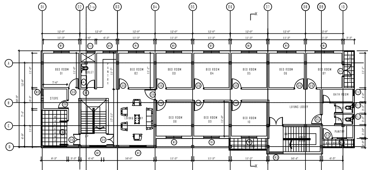
FIRST FLOOR PLAN (3072.22 square ft.)
