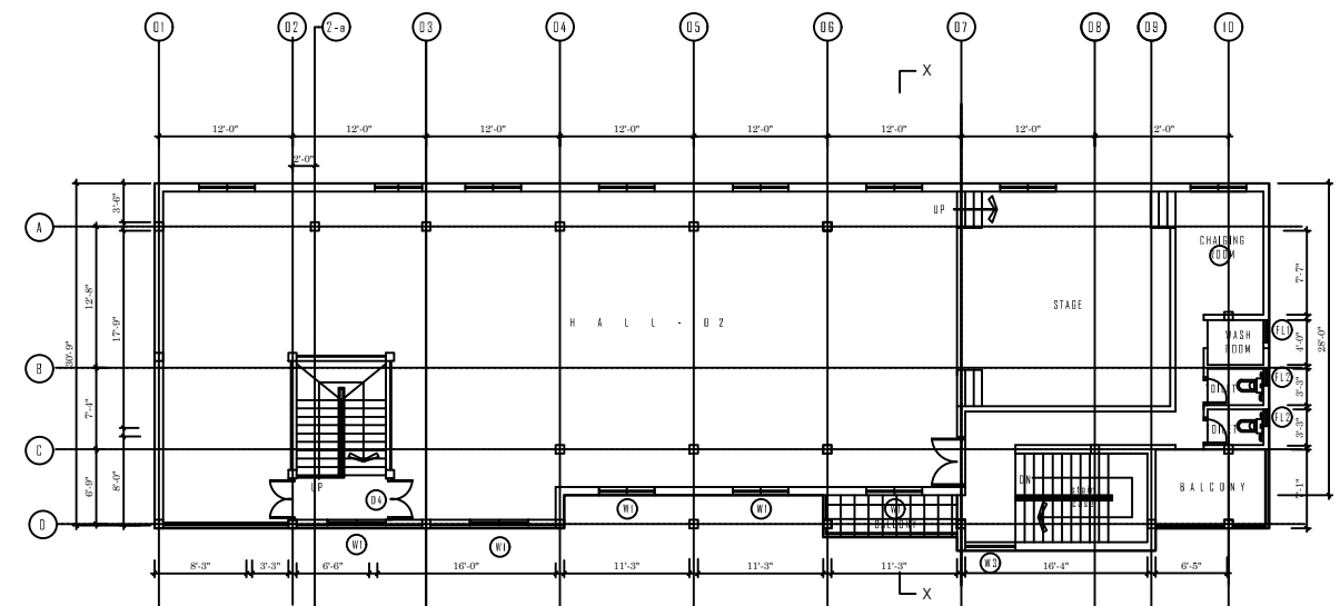
third floor plan (3072.22 square ft.)
