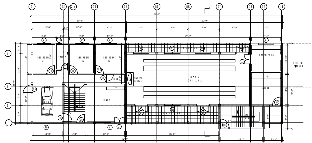
GROUND FLOOR PLAN (2984.47 square ft)
