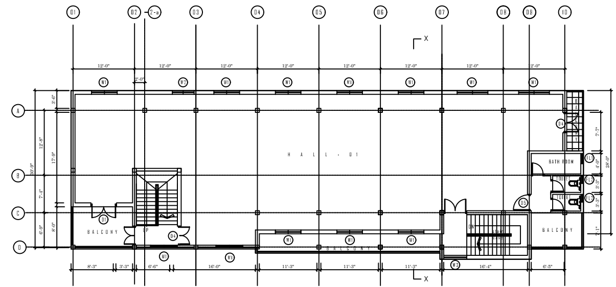
SECOND FLOOR PLAN (3160.00 square ft.)
